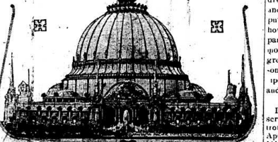
Copyright, 1914, by Panama Pacific International Exposition Company. The superb Palace of Horticulture at the Panama-Pacific International exposition in San Francisco will be surrounded by a vast dome of glass, supported with immense steel struts. The dome will be 136 feet in height, of 122 feet in diameter. At night batteries of colored searchlights will play on the inside of the dome from within, so that it will present the appearance of a gigantic soap bubble continuously changing to every color of the rainbow.
