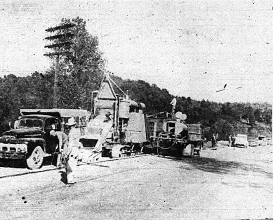
The large mixer being used to lay down the concrete truck lane through the "Big Cut". Approximately one mile of the lane is finished. Another breakdown of the machinery last Monday is causing serious delay.
