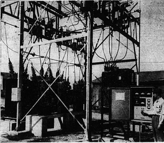
Roy B. Owens, local Kentucky Utilities Company manager, is shown at the panel of the automatic reclosing oil circuit breakers installed at the Mt. Vernon substation of the electric company. In the left foreground are the three newly installed voltage regulators. The substation was rebuilt to improve electric service here.
