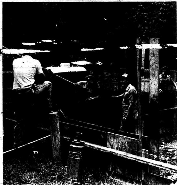
Current renovation of the Mt. Vernon city sewer plan includes rebuilt and some new drying beds, a new center column and pipe arms and a rebuilt comminutor. The renovation is expected to be $28,056 most of which will be offset by a construction grant from area development funds. Some of the work is being done by city employees and some by David Shivel, general contractor. In the above photo, from left, are Shivel and three employees of Tucker Concrete of Bronston, Ky. Tucker poured the concrete on the
