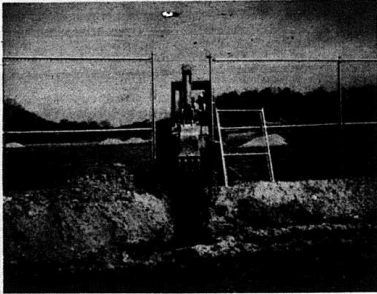
Harris Construction of London is shown installing the drainage system in the ballfield area of Lake Linville. The project includes the installation of drainage tile and a rock filter. Construction will be completed during May, 1985.
