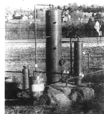
Hunt's Scrubber which collects the gas and makes sure it is clean before sending under the road is located across the bypass.
