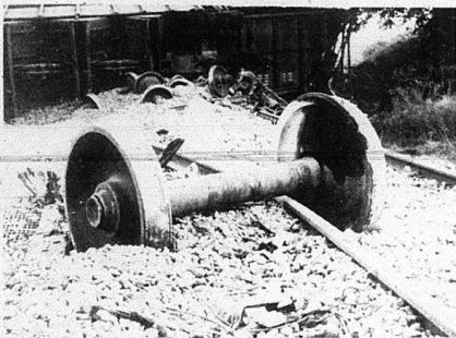
Preliminary investigation of the five-car derailment at Roundstone near Parsons Gas last Friday, indicates the axle at left may have broken causing the accident.
